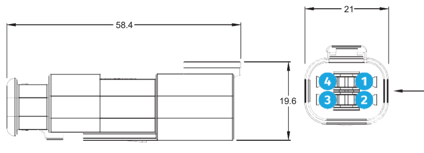
MALE (ATM)
