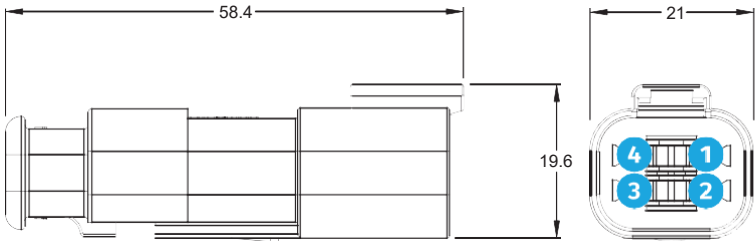
MALE (ATM)
